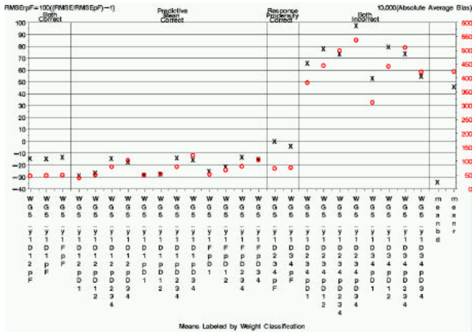
Figure 1: RMSErF and AB by Model Correctness; Simulation I
