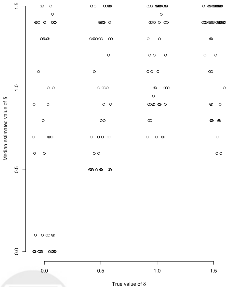
Figure 3: Median estimated values of \delta for the simulation study across the remaining simulation parameters, with J = 8 and G = 1,000 by the the true value used for simulation.
