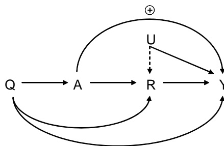
Fig. 1. Motivating example concerning the estimation of controlled direct effects.
