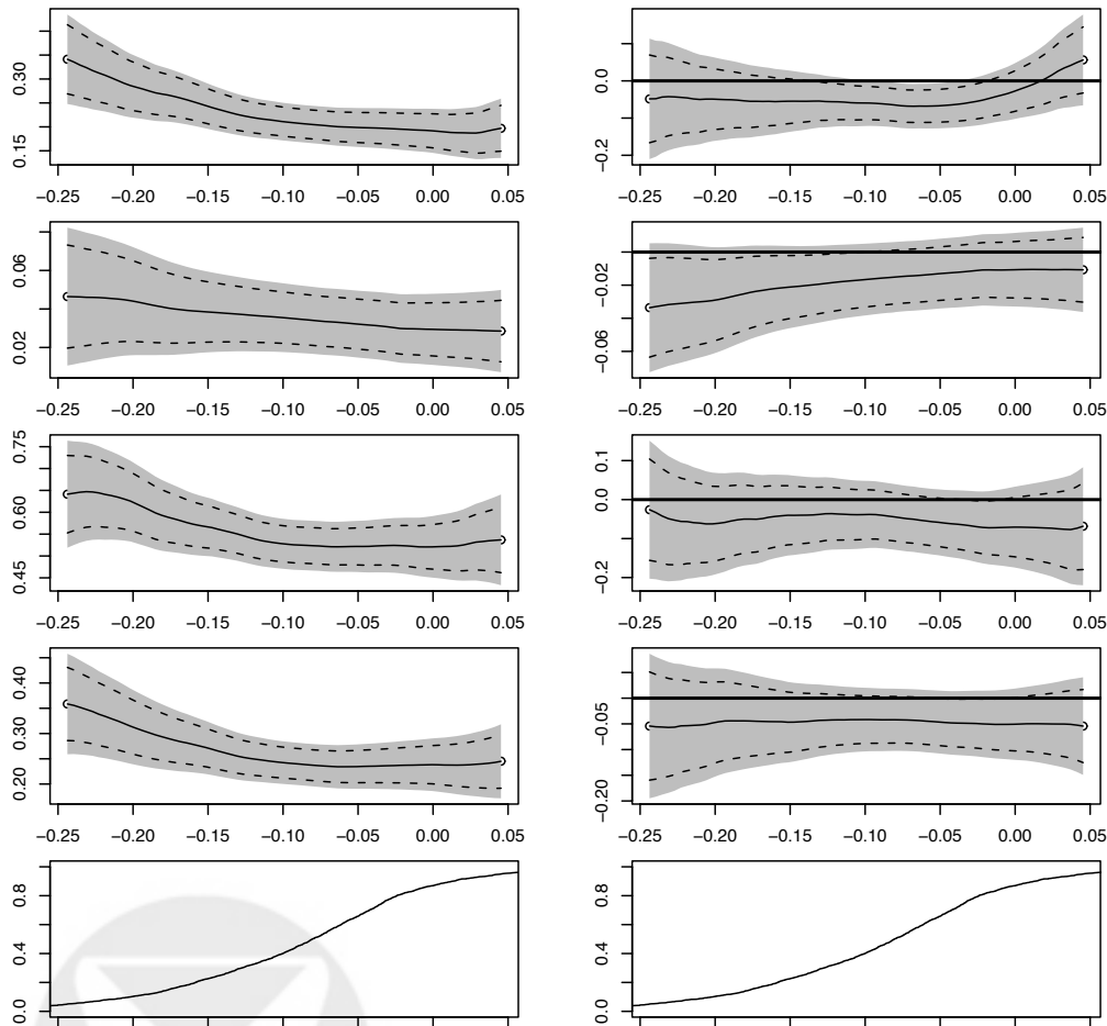
Figure 3: Use of \hat{\pi}_2(U) - \hat{\pi}_1(U) as a scoring system (left panel: 1.5-year event probabilities in control group; right panel: 1.5-year treatment effect; from top: death, MI, hospitalization, AE discontinuation; bottom row: empirical CDF of risk scores).
