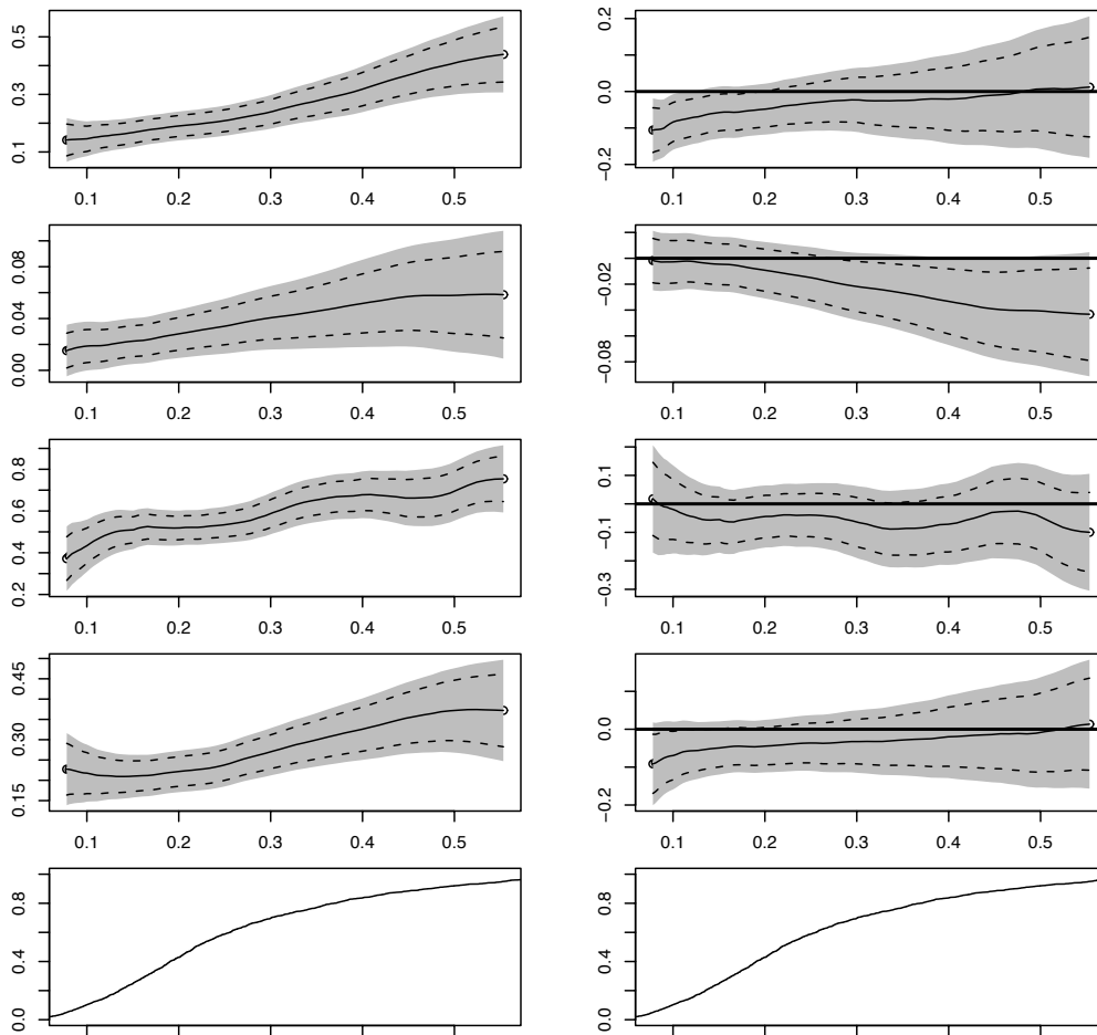
Figure 2: Use of \hat{\pi}_1(U) as a scoring system (left panel: 1.5-year event probabilities in control group; right panel: 1.5-year treatment effect; from top: death, MI, hospitalization, AE discontinuation; bottom row: empirical CDF of risk scores).
