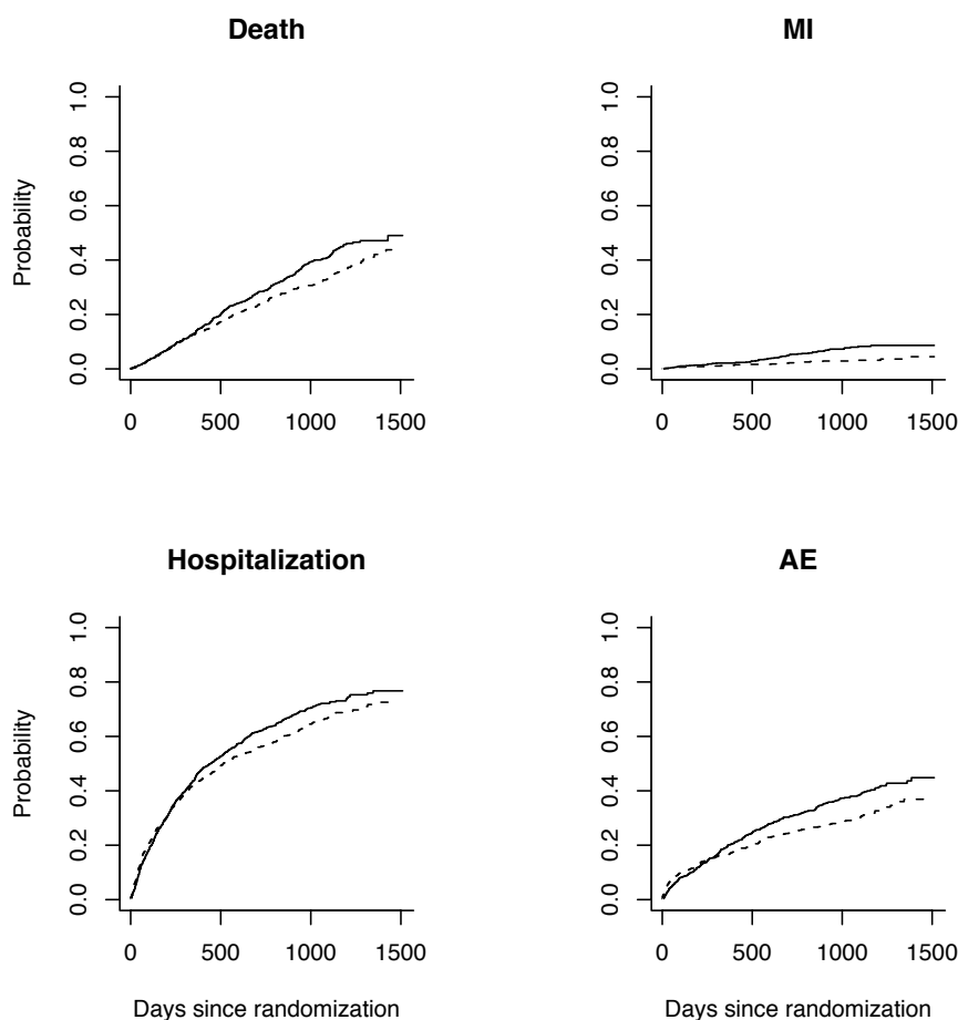
Figure 1: Cumulative incidence function estimates for each endpoint (solid: control group, dashed: treated group).
