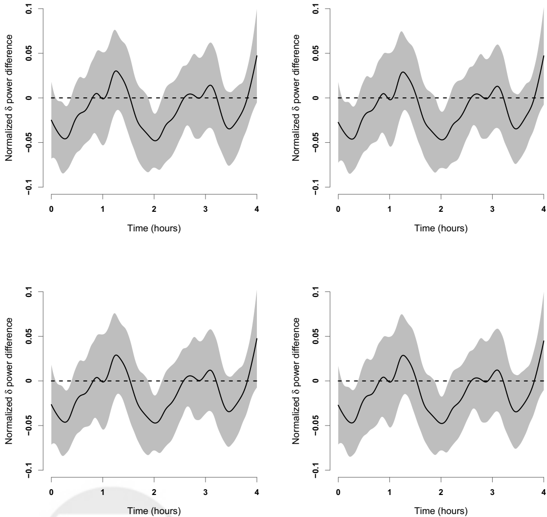
Figure 3: Mean difference and 95% pointwise confidence intervals via the parametric bootstrap. Top-left panel: results for K = 36 and L = 26 chosen such that 90% of the variability described by K^X(\cdot, \cdot) and K^U(\cdot, \cdot) is explained. We also used the standard estimator of the variability, \sigma_\epsilon . Top-right panel: explained variability is increased to 95% ( K = 49 , L = 40 ) with the same estimator of \sigma_\epsilon . Left-bottom panel: explained variability is 95% with an estimator that is roughly 20% larger than the standard estimator. Right-bottom panel: explained variability is 99% ( K = 76 , L = 69 ) at both levels with the same conservative estimator of \sigma_\epsilon .
