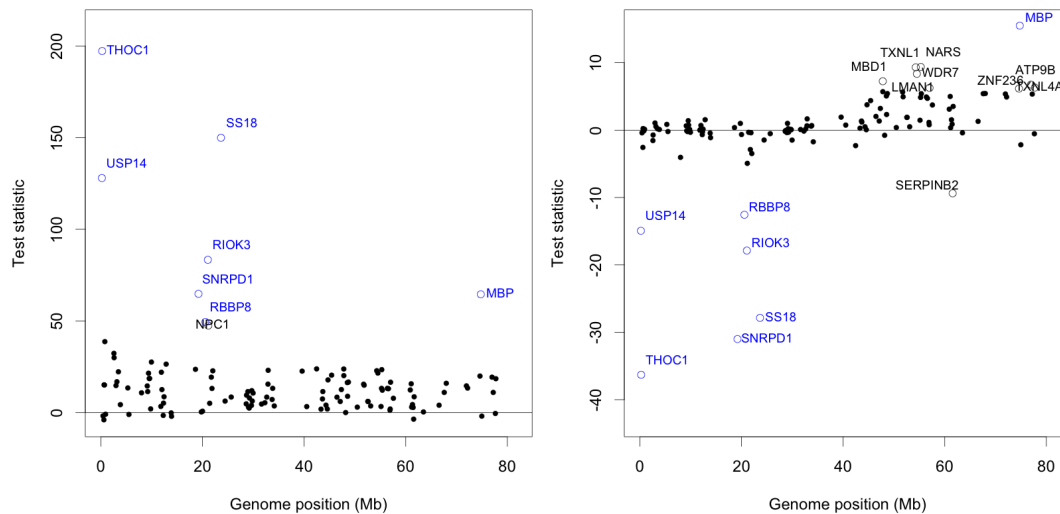
Figure 4: Real data application to the 130 genes of chromosome 18 in the OvCa dataset (ovarian cancers). We represent the tests statistics \sqrt{n}(\psi_n^{g,3} - \psi_{\text{ref}}^g)/s_n^{g,3} for \psi_{\text{ref}}^g = 0 (left graphic) and \psi_{\text{ref}}^g = \mathcal{F}(P_n^g) (right graphic) along the position of gene g on the genome. We report the names of the genes such that \sqrt{n}|\psi_n^{g,3}|/s_n^{g,3} > 45 (left graphic) and \sqrt{n}|\psi_n^{g,3} - \mathcal{F}(P_n^g)|/s_n^{g,3} > 6 (right graphic), the cut-offs being arbitrarily chosen.
